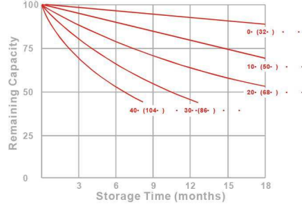
Capacity Retention Characteristic
