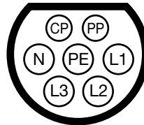
(b) 3-phase type 2 plug
