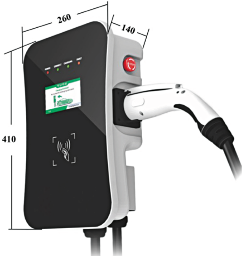
Fig. 4-1 The Shape & Dimensions of M3W
